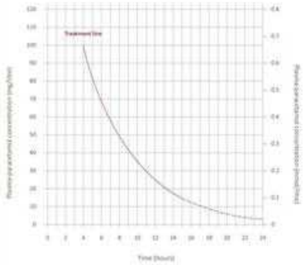
Fig 2.20 Paracetamol overdose treatment nomogram.
