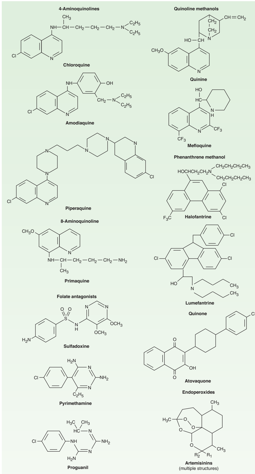
FIGURE 52-2 Structural formulas of antimalarial drugs.
