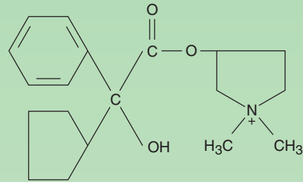
Glycopyrrolate
