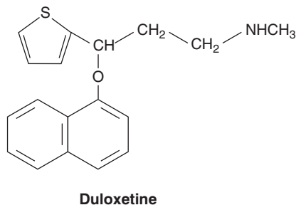
Duloxetine
